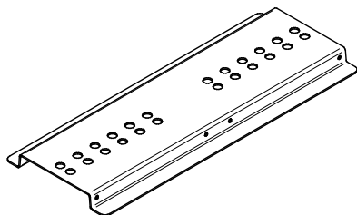
JONCTION DE MONTANT VERTICAL (K) FINISHING TRIM JUNCTION 2X PL77352
