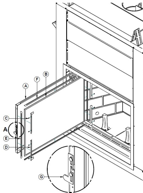
DETAIL A
