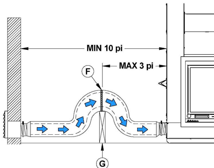
Figure 5 : P-Trap Example
