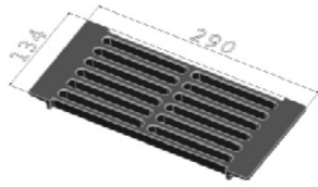
Grate PST-1001-305 (1)
